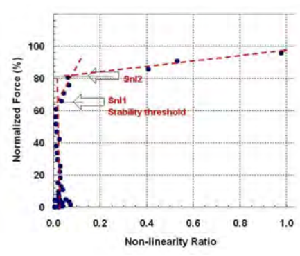
(5c) Non-linearity based technique
