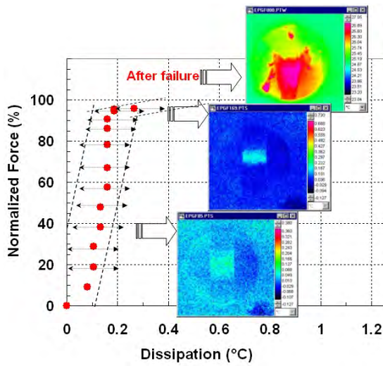
(4a) Quasi homogeneous diorite D.
