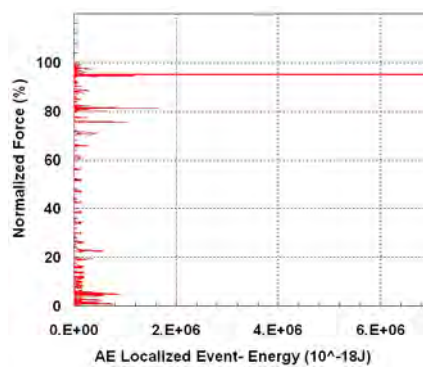
(5b) AE based technique
