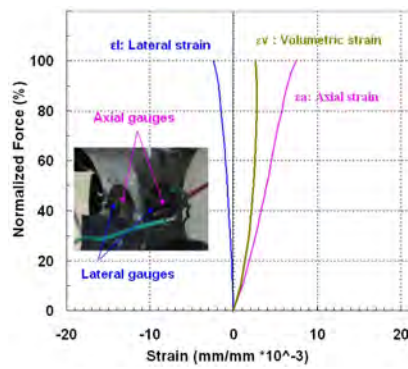
(5a) Strain based technique
