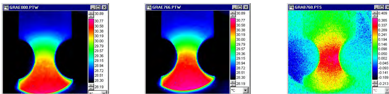
(2a) Thermogram recorded at reference load level. (2b) Thermogram recorded at a given load level. (2c) = Thermogram (2b) – Thermogram (2a).
