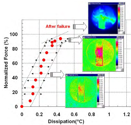
(4b) Heterogeneous granite G.
